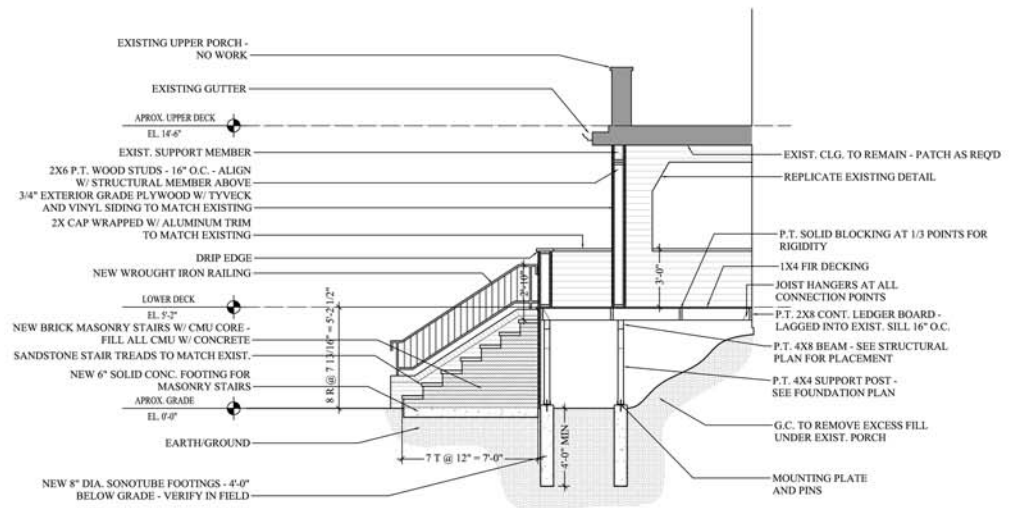
Construction Section
